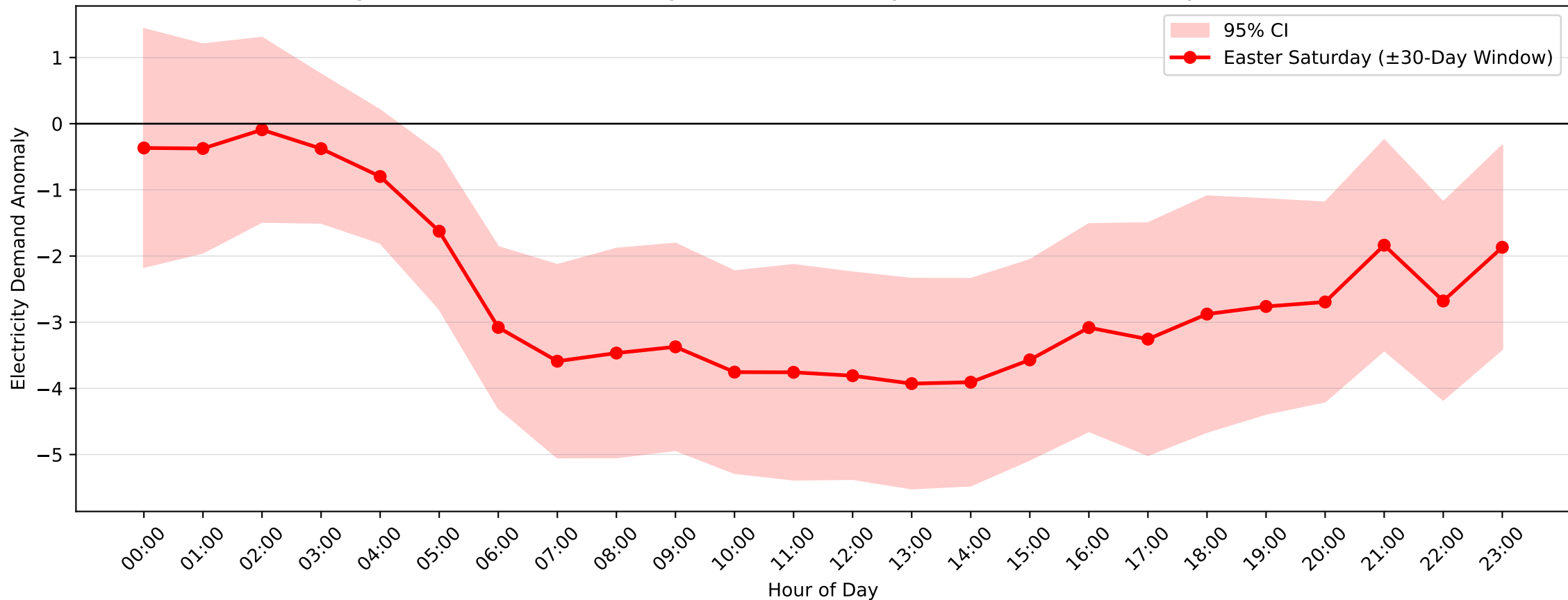
Argenton Demand Anomaly: Easter Saturday (2004-2017, \pm 30 -Day Window)
